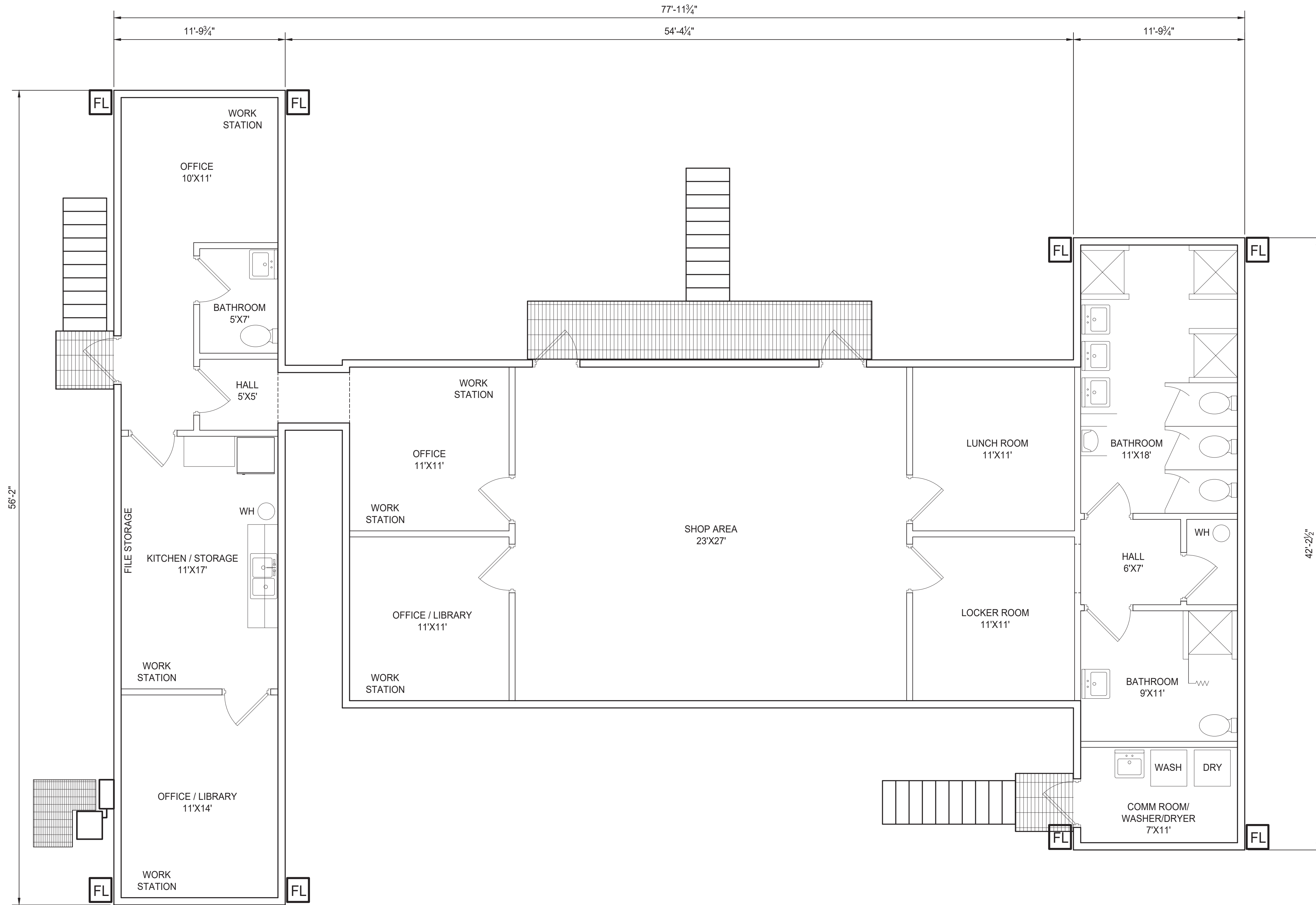
ADMINISTRATION BUILDING FLOOR AND LIGHTING PLAN BUILDING FLOOR AREA = 2390 SQUARE FEET SCALE 1/4" = 1'-0"
