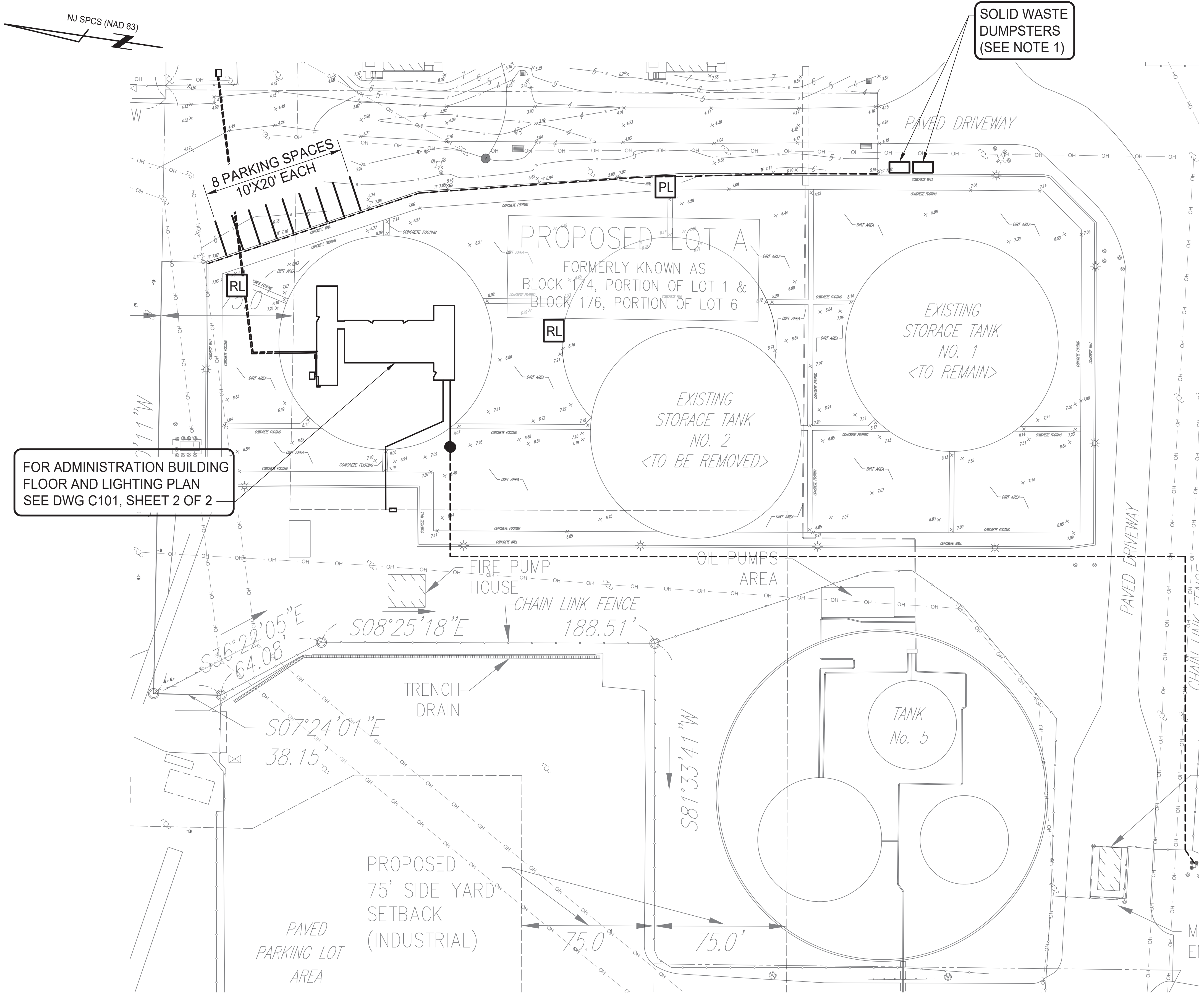
SITE PARKING AND LIGHTING PLAN SCALE 1"=30'
