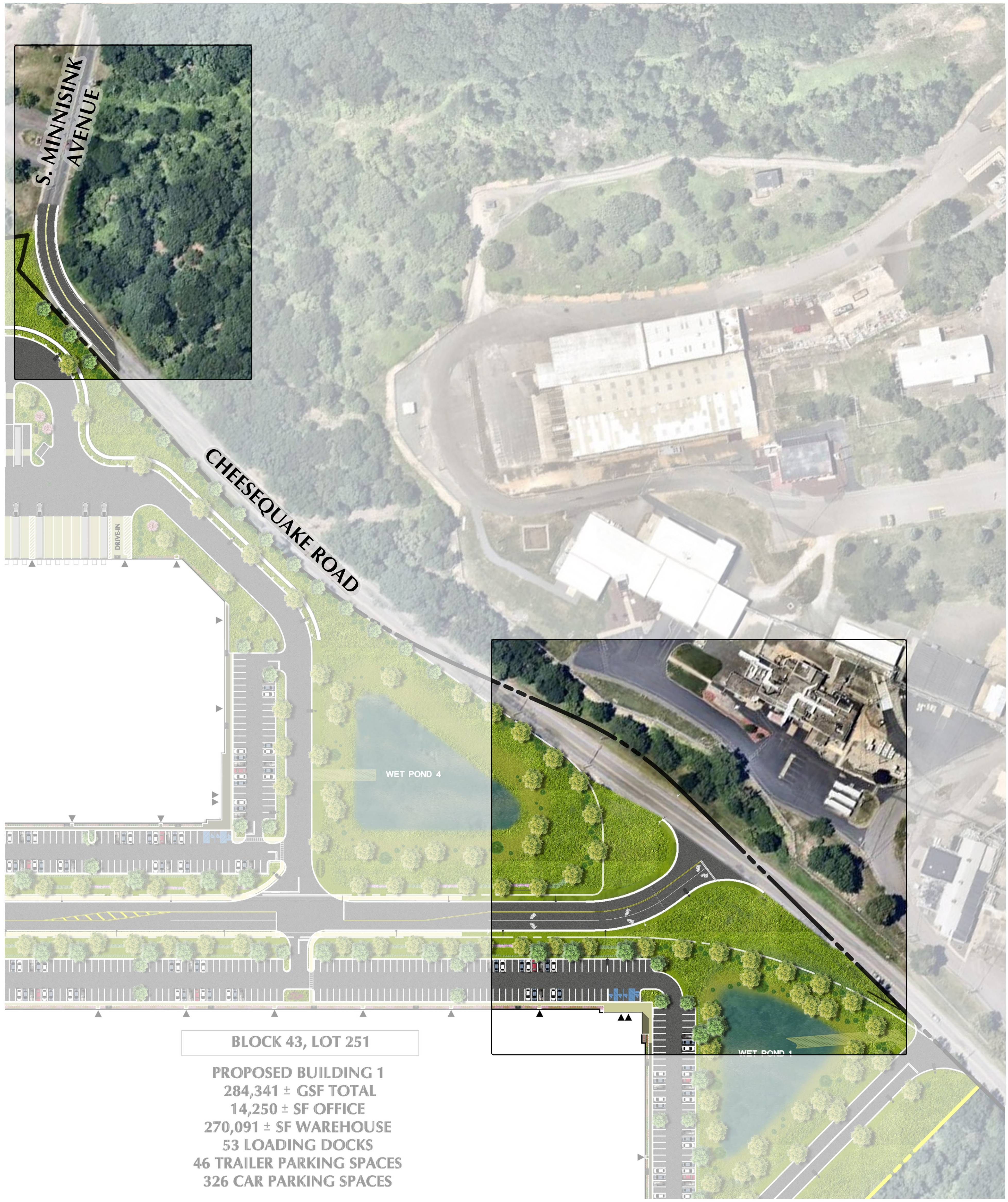
INTERIM ROADWAY GEOMETRY
