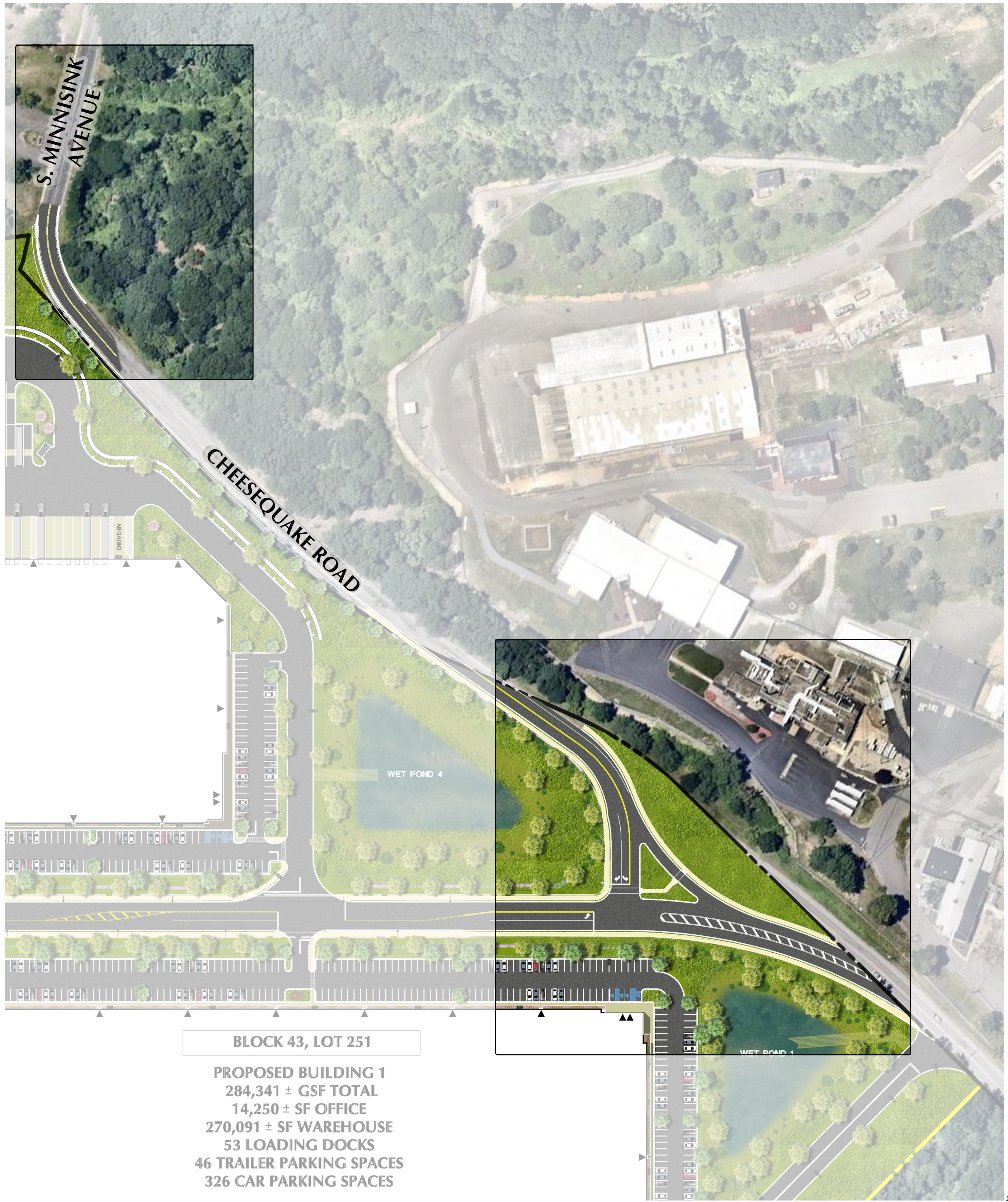
FINAL INTERSECTION ROADWAY GEOMETRY
