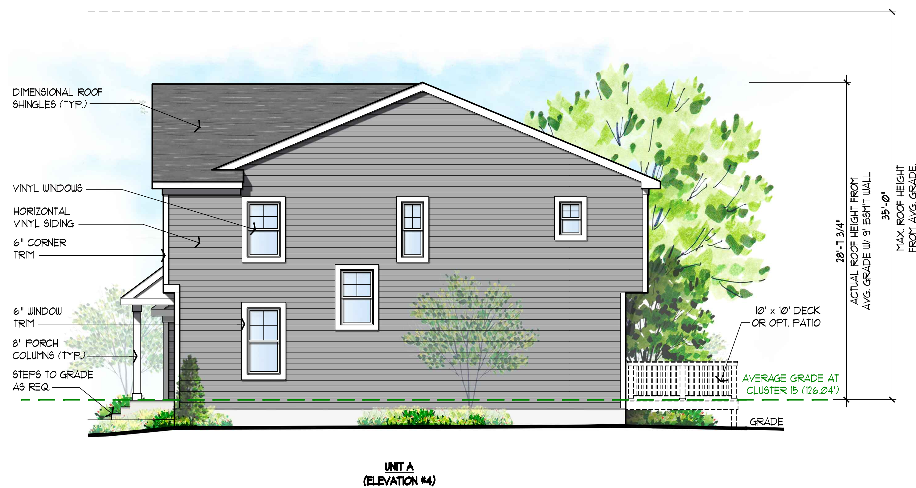
RIGHT SIDE ELEVATION (6-UNIT BUILDING)
