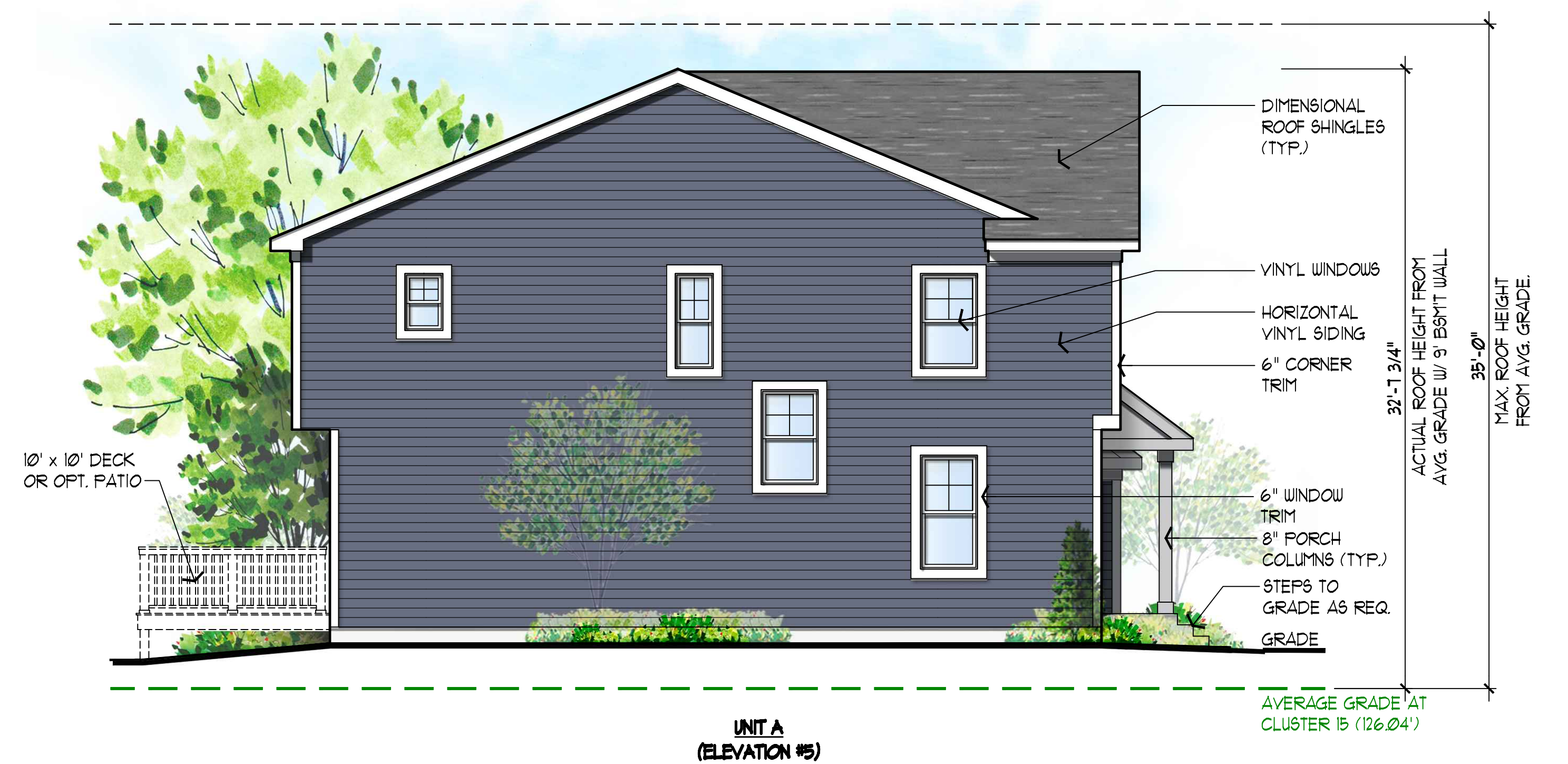
LEFT SIDE ELEVATION (6-UNIT BUILDING)
